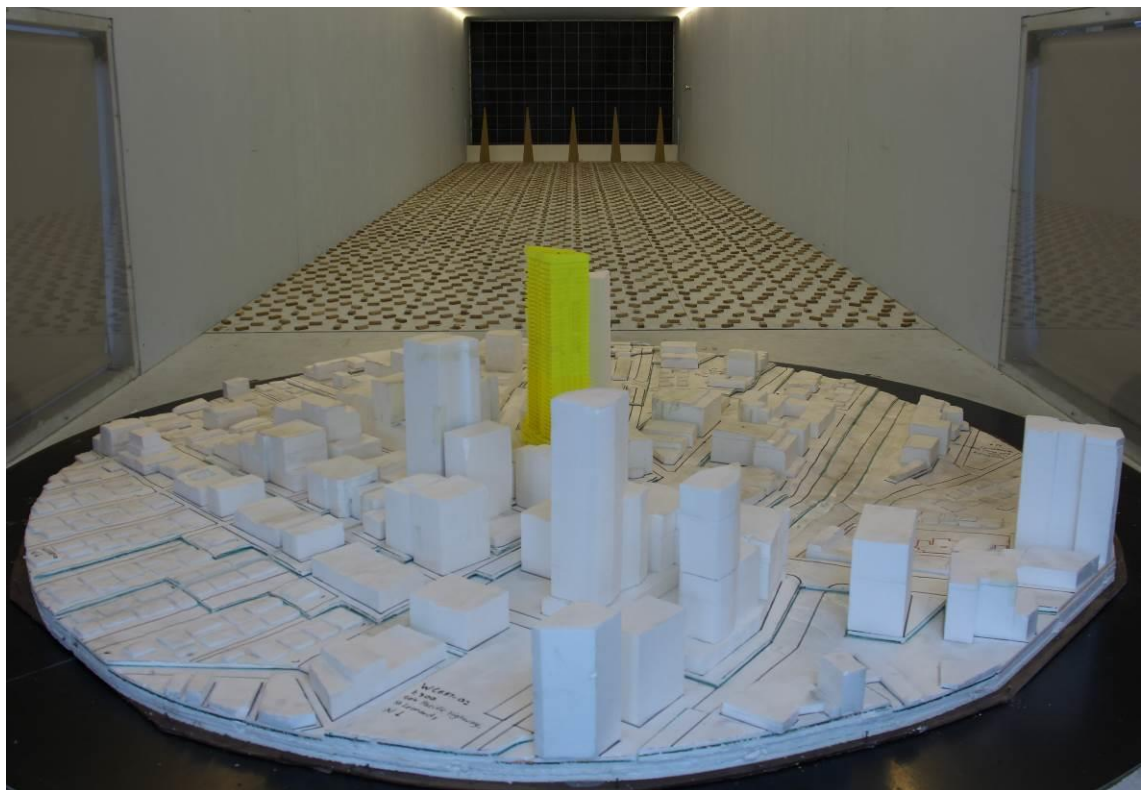
Figure 2o: Photograph of the Wind Tunnel Model – Proposed Development with the Proposed 472-486 Pacific Highway Development – View from the North-West
