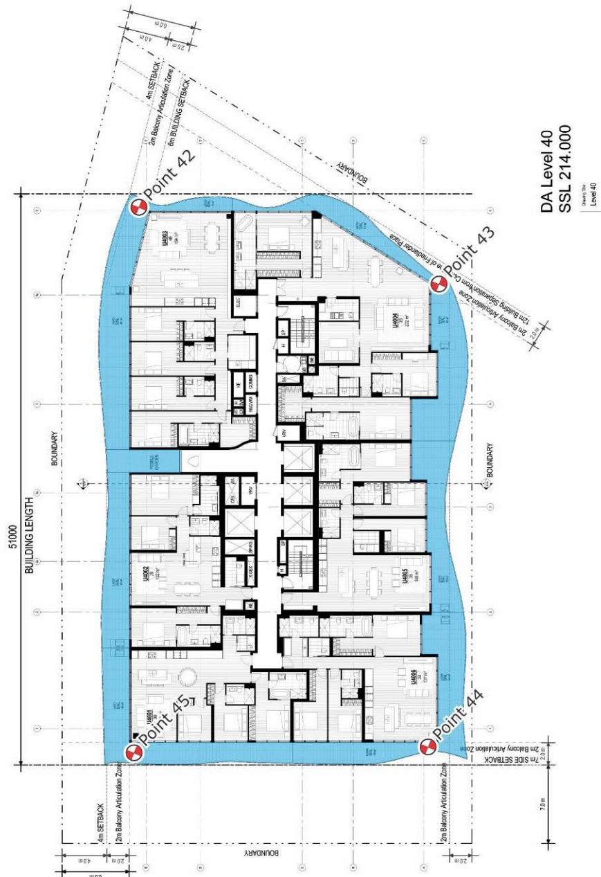
Figure 5i: Study Point Locations and Target Criteria – Level 40
