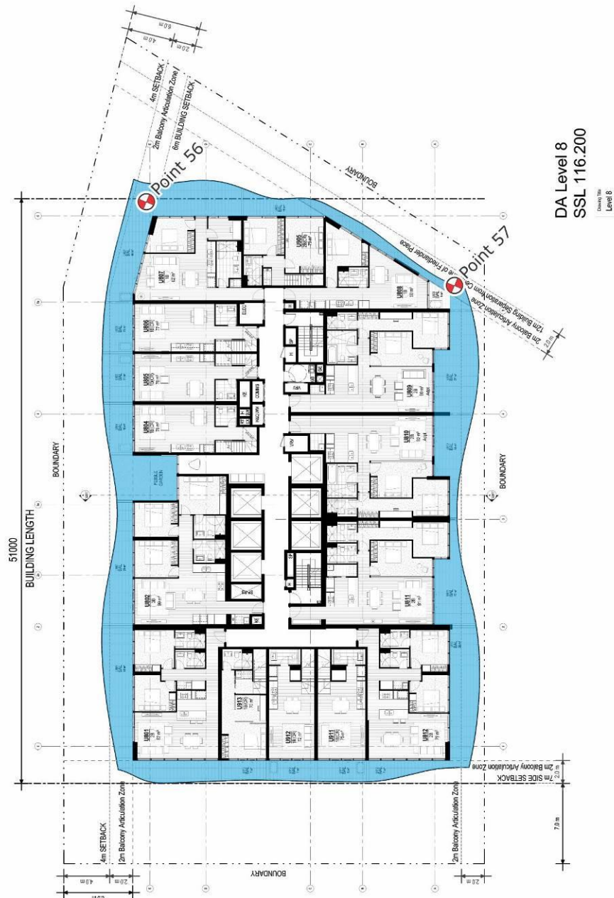
Figure 5g: Study Point Locations and Target Criteria – Level 8
