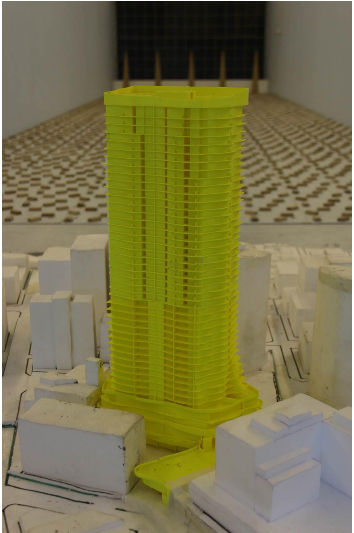
Figure 2i: Photograph of the Wind Tunnel Model – Proposed Development with the Existing 472-486 Pacific Highway Development – View from the South
