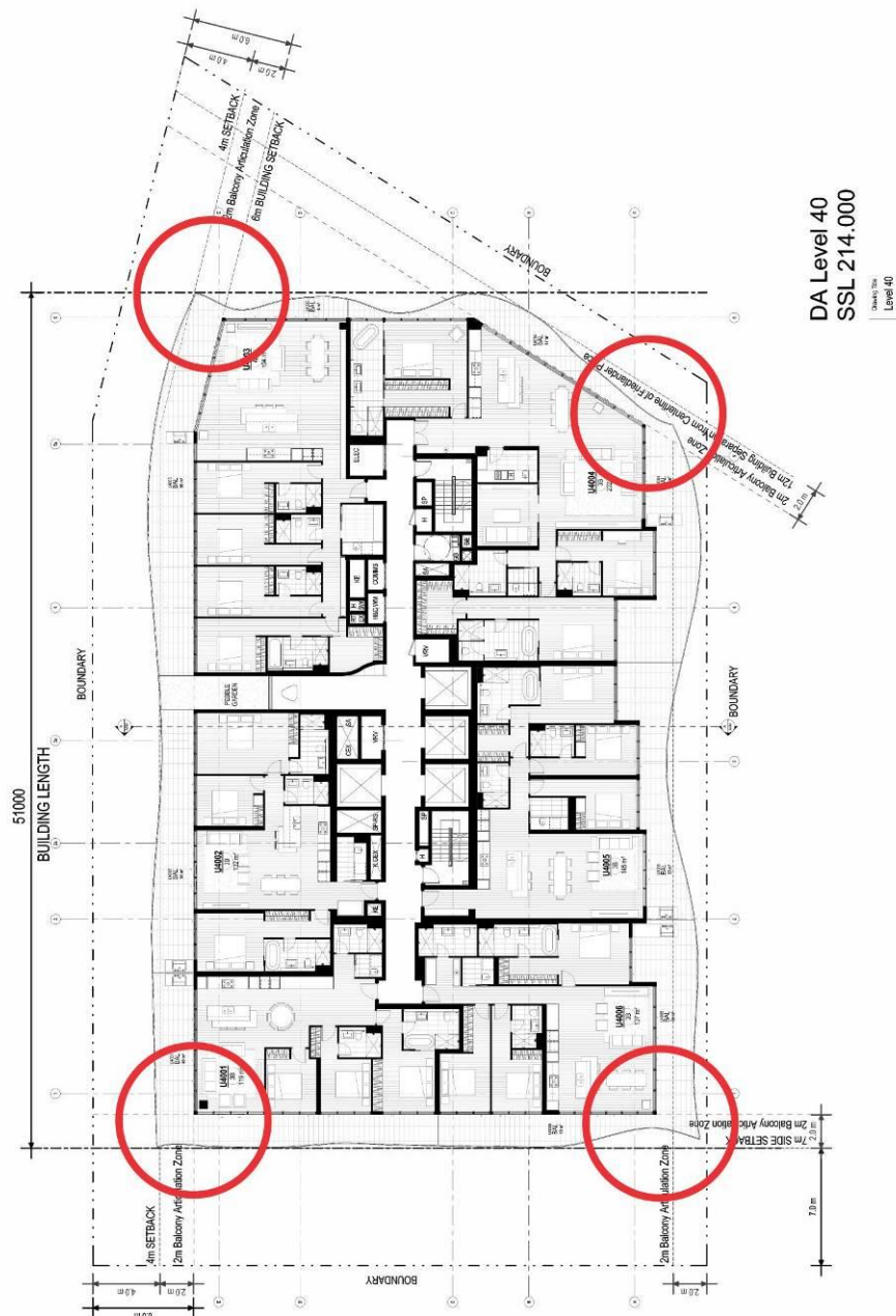
Figure 8h: Recommended Treatments on Level 26-43
