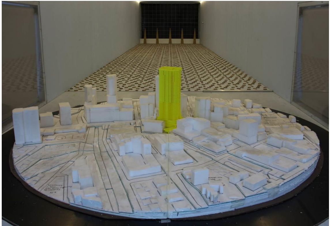
Figure 2a: Photograph of the Wind Tunnel Model – Proposed Development with the Existing 472-486 Pacific Highway Development – View from the South
