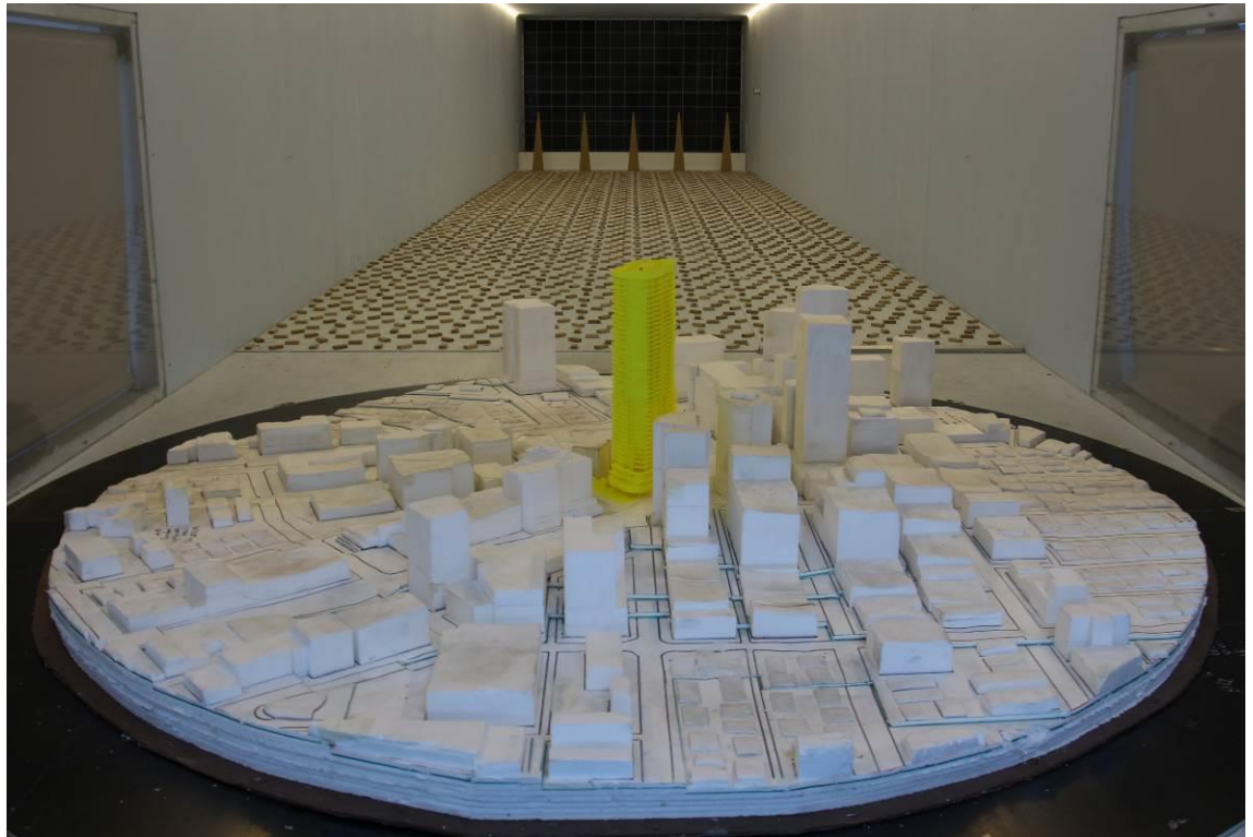
Figure 2c: Photograph of the Wind Tunnel Model – Proposed Development with the Existing 472-486 Pacific Highway Development – View from the East
