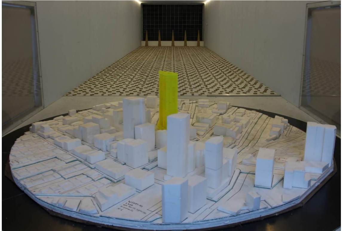
Figure 2f: Photograph of the Wind Tunnel Model – Proposed Development with the Existing 472-486 Pacific Highway Development – View from the North-West
