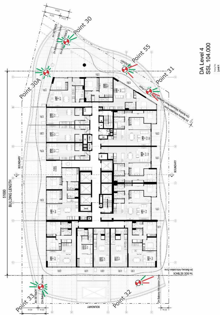
Figure 6g: Wind Directionality Plots – Level 4 - Proposed Development with the Existing 472-486 Pacific Highway Development (results shown without any treatments applied)
