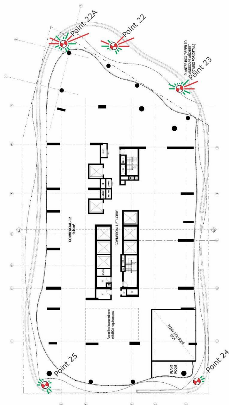
Figure 6e: Wind Directionality Plots – Level 2 - Proposed Development with the Existing 472-486 Pacific Highway Development (results shown without any treatments applied)
