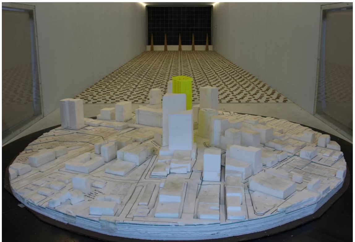
Figure 2k: Photograph of the Wind Tunnel Model – Proposed Development with the Proposed 472-486 Pacific Highway Development – View from the South-East
