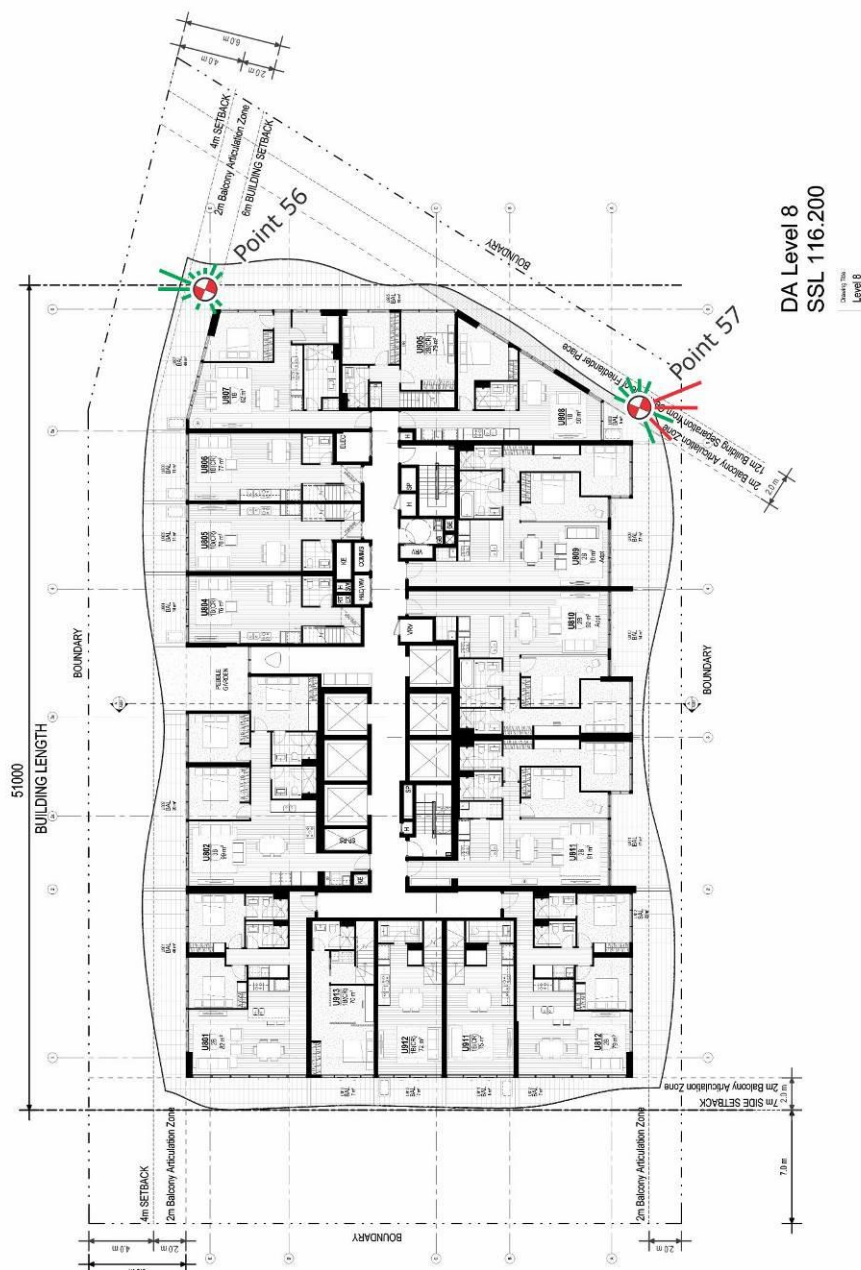
Figure 7i: Wind Directionality Plots – Level 8 - Proposed Development with the Proposed 472-486 Pacific Highway Development (results shown without any treatments applied)
