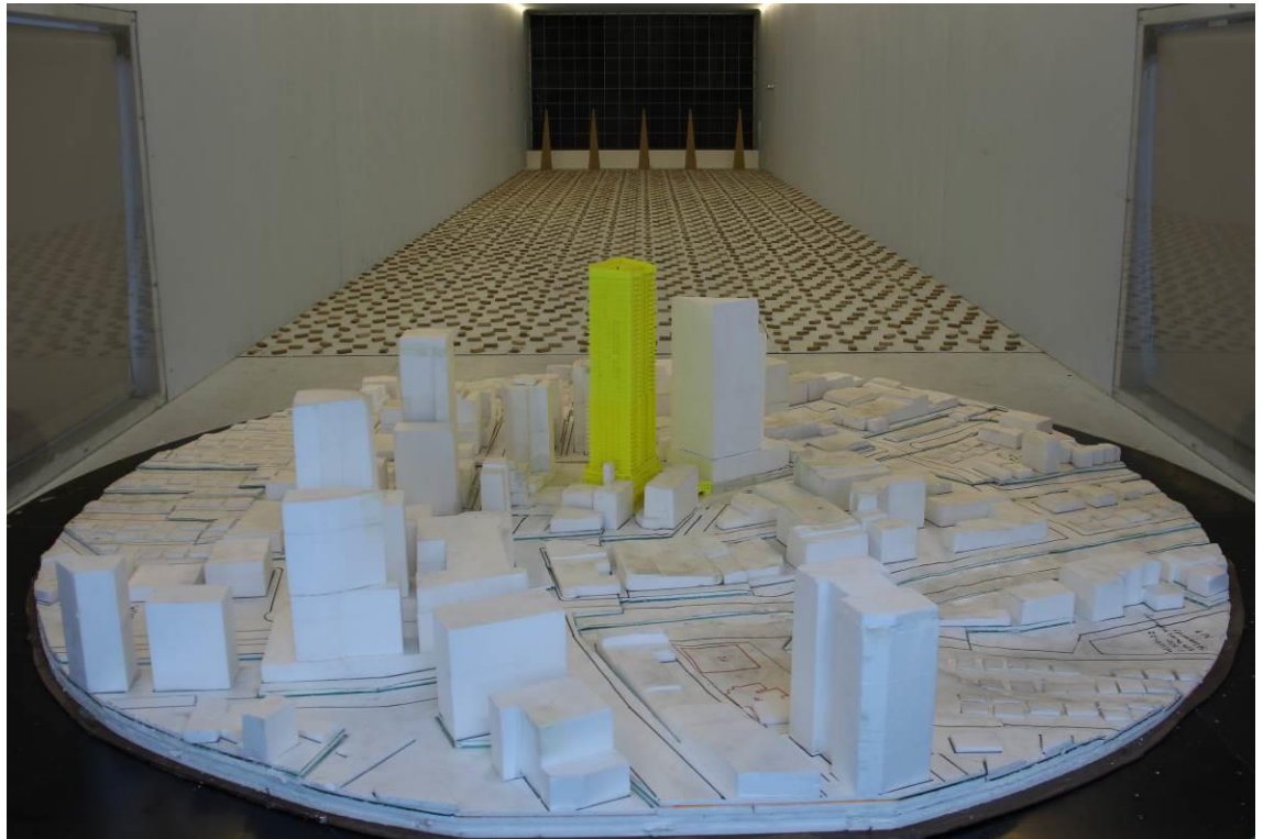
Figure 2p: Photograph of the Wind Tunnel Model – Proposed Development with the Proposed 472-486 Pacific Highway Development – View from the West
