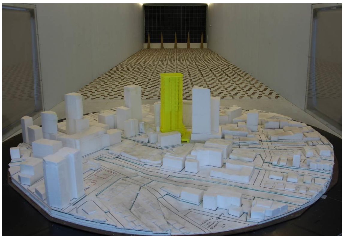
Figure 2q: Photograph of the Wind Tunnel Model – Proposed Development with the Proposed 472-486 Pacific Highway Development – View from the South-West
