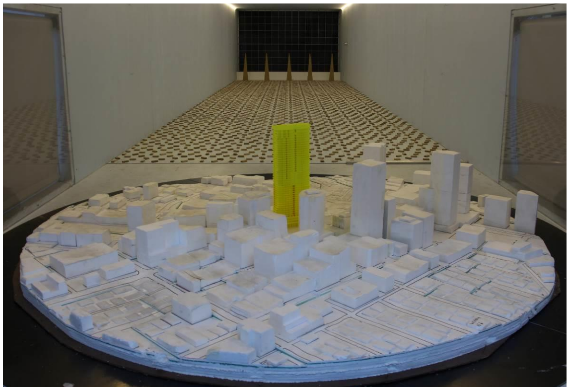
Figure 2d: Photograph of the Wind Tunnel Model – Proposed Development with the Existing 472-486 Pacific Highway Development – View from the North-East
