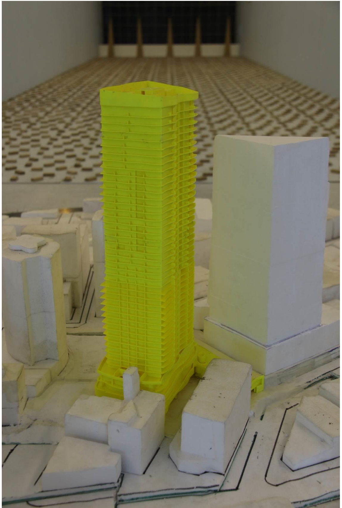
Figure 2r: Photograph of the Wind Tunnel Model – Proposed Development with the Proposed 472-486 Pacific Highway Development – View from the West
