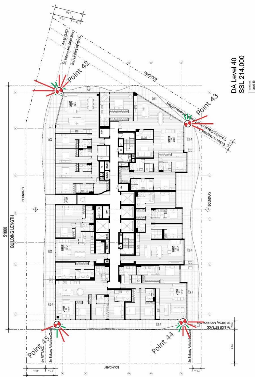
Figure 6k: Wind Directionality Plots – Level 40 - Proposed Development with the Existing 472-486 Pacific Highway Development (results shown without any treatments applied)
