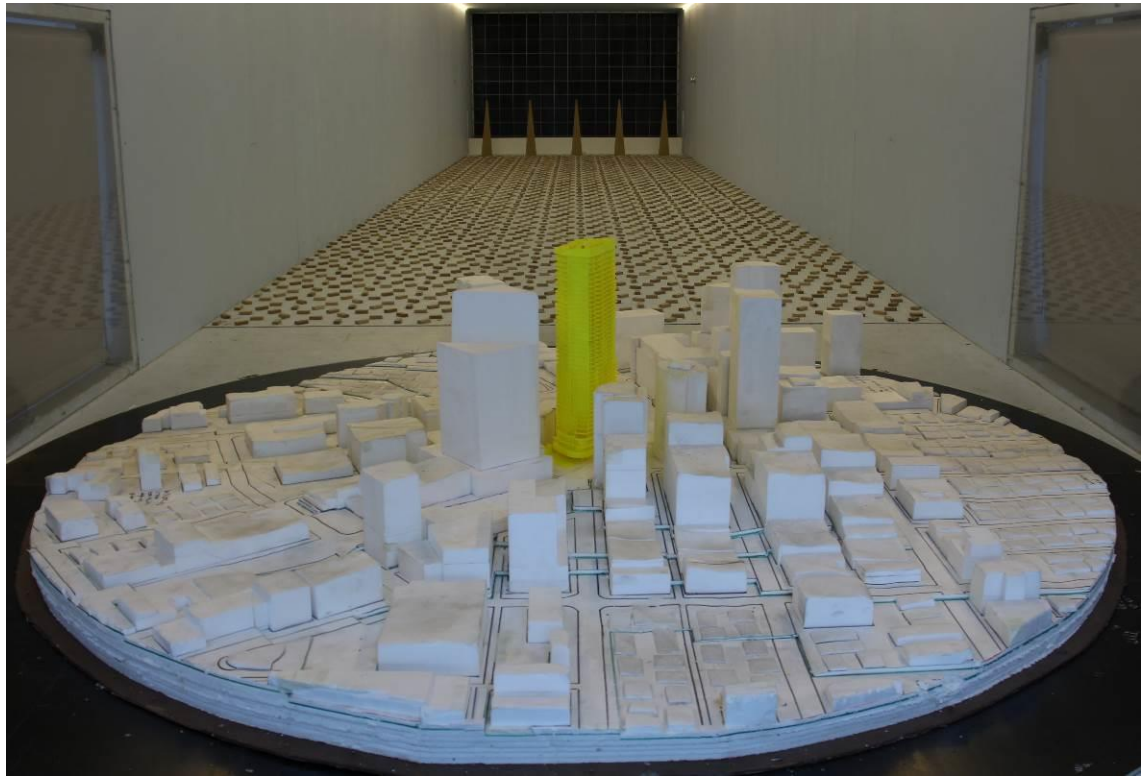
Figure 2l: Photograph of the Wind Tunnel Model – Proposed Development with the Proposed 472-486 Pacific Highway Development – View from the East
