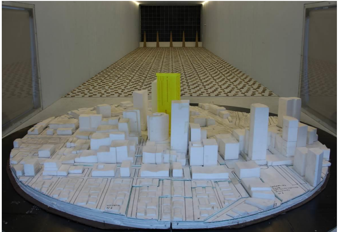
Figure 2n: Photograph of the Wind Tunnel Model – Proposed Development with the Proposed 472-486 Pacific Highway Development – View from the North
