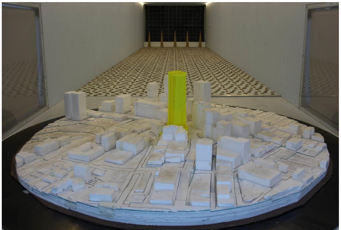
Figure 2b: Photograph of the Wind Tunnel Model – Proposed Development with the Existing 472-486 Pacific Highway Development – View from the South-East
