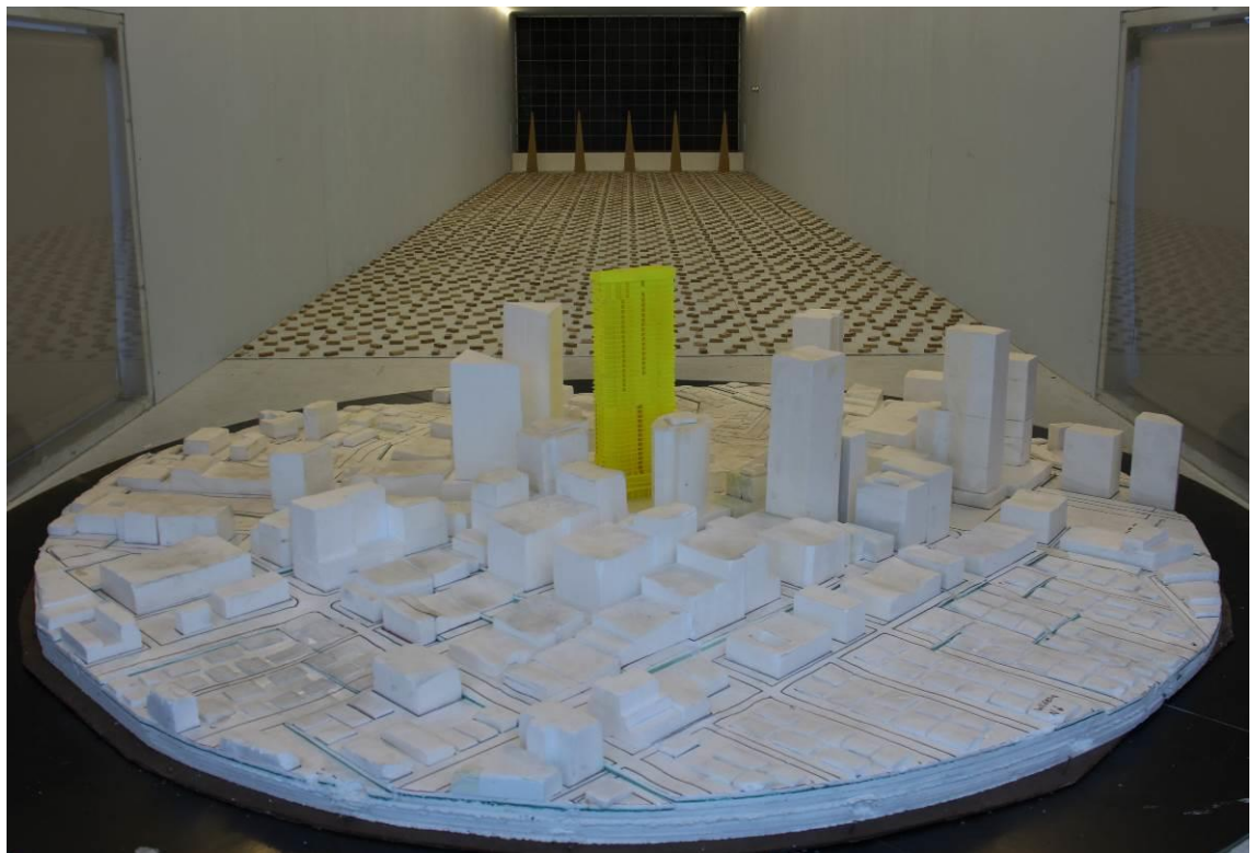
Figure 2m: Photograph of the Wind Tunnel Model – Proposed Development with the Proposed 472-486 Pacific Highway Development – View from the North-East
