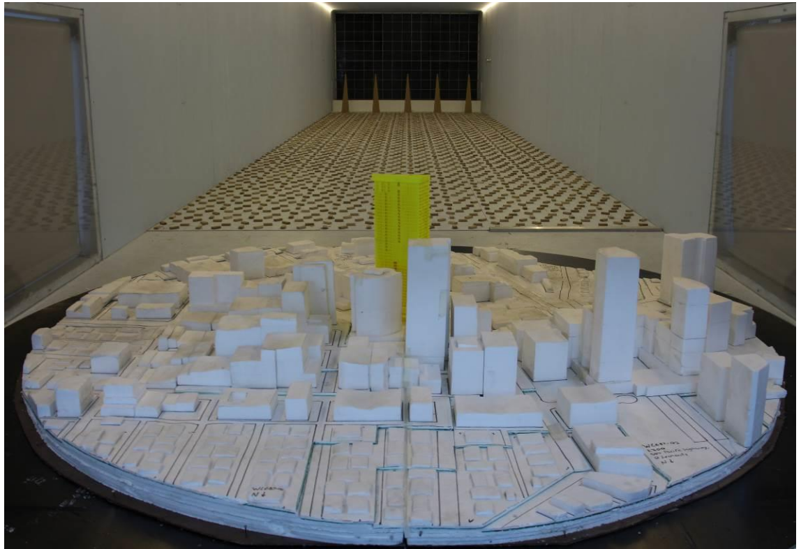
Figure 2e: Photograph of the Wind Tunnel Model – Proposed Development with the Existing 472-486 Pacific Highway Development – View from the North
